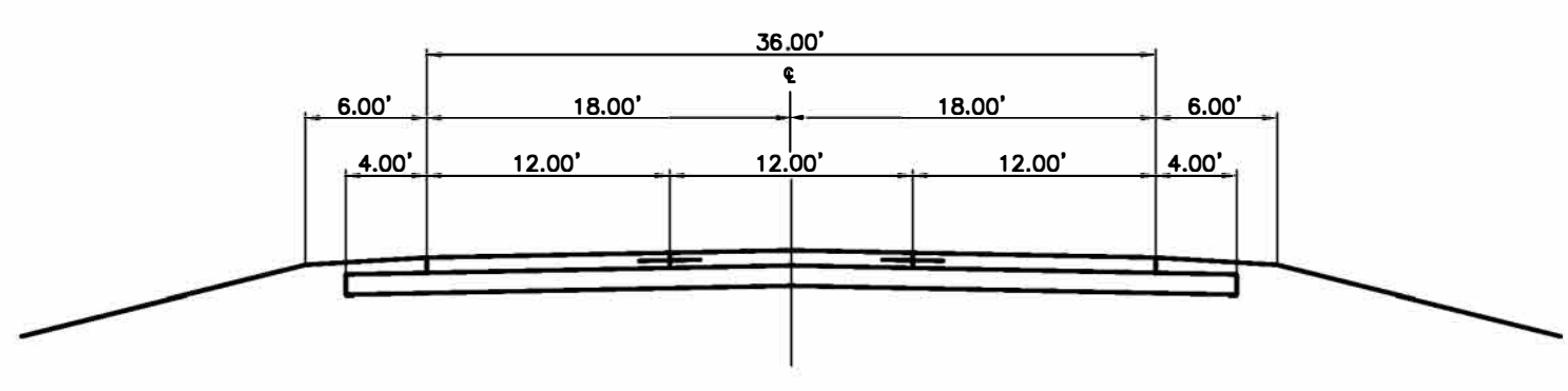
TYPICAL SECTIONS - CORNHUSKER ROAD B-B SECTION NO SCALE
